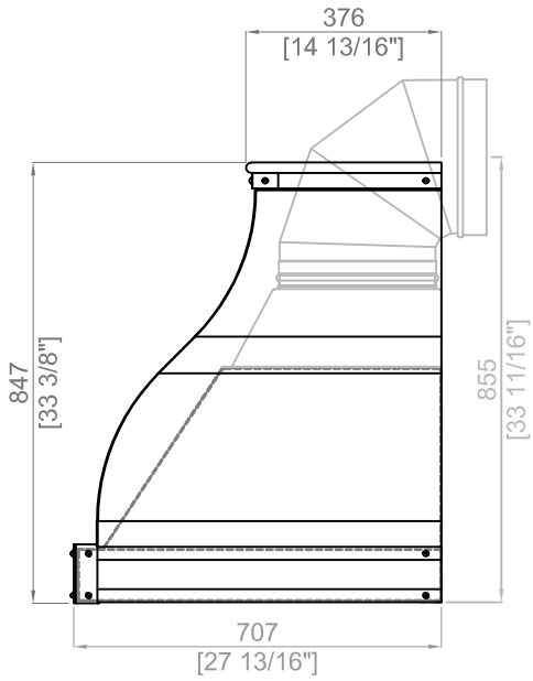
BACK VENTING
