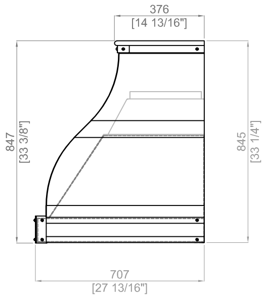
TOP VENTING
