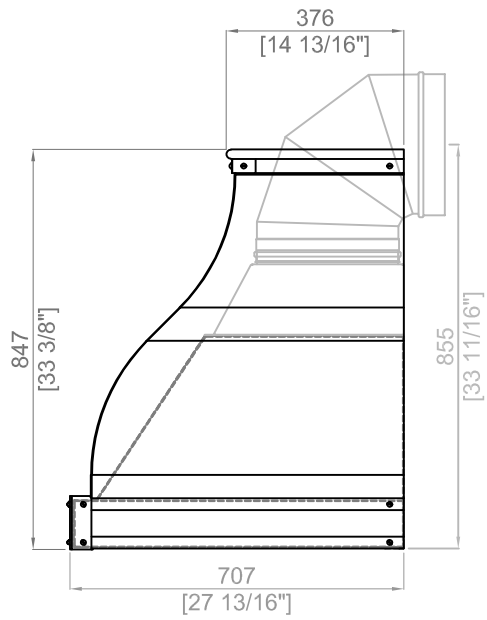
BACK VENTING
